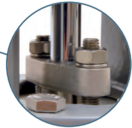
Easy access adjustable gland pack
