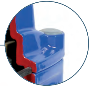
Polymere hat screws for anti-corrosion protection
