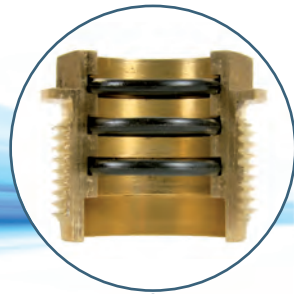
Stem tightness with 3 NBR O-ring gaskets
